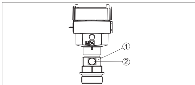
Fig. 8: Position of the filter element - Ex d version
