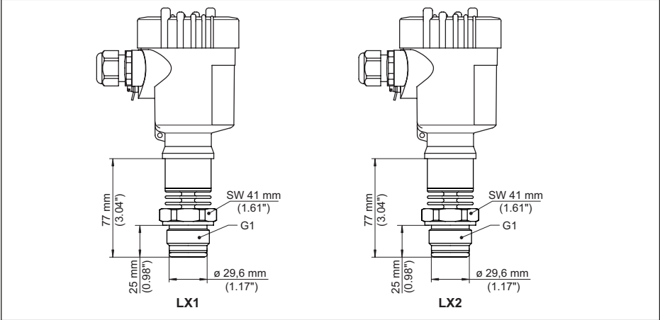
Fig. 44: VEGABAR 83, thread for hygienic adapter
