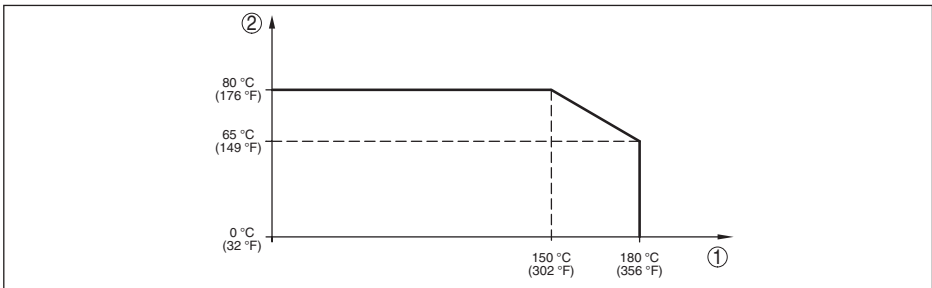
Fig. 37: Temperature derating VEGABAR 83, version up to +180 °C (+356 °F)
