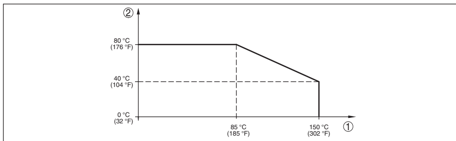
Fig. 35: Temperature derating VEGABAR 83, version up to +150 °C (+302 °F)
