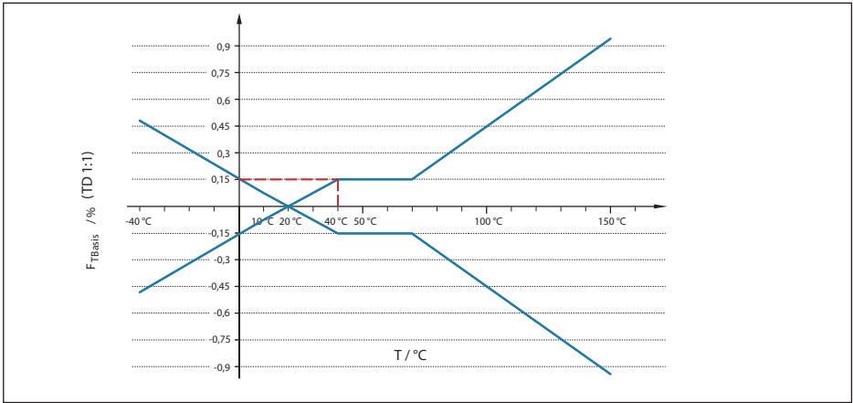
Fig. 39: Determination of the basic temperature error for the above example: F_{\text{TBasis}} = 0.15 \%
